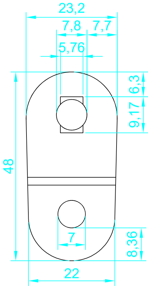
Face of Switch
